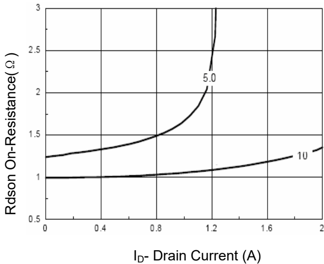
Figure 3 Drain-Source On-Resistance
