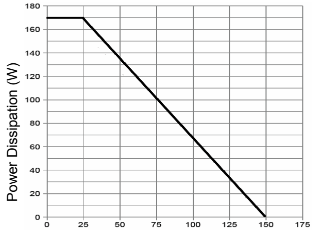
T J -Junction Temperature(°C) Figure 8 Power De-rating
