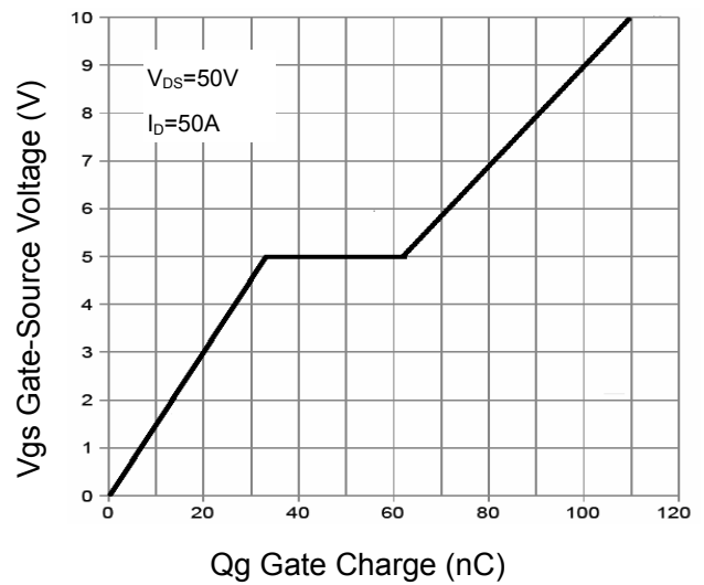
Figure 4 Gate Charge
