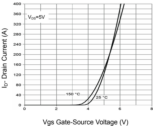
Figure 3 Transfer Characteristics
