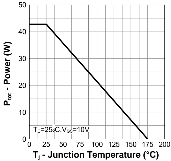
Power Capability
