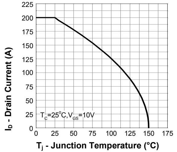
Current Capability
