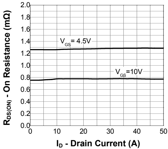
On Resistance
