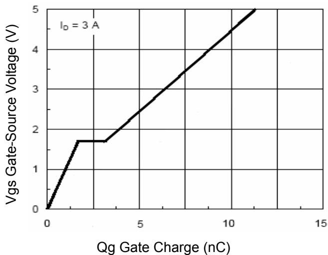
Figure 5 Gate Charge
