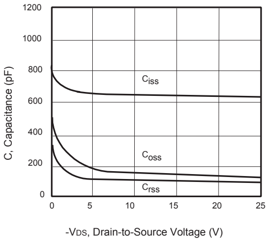
Figure 3. Capacitance
