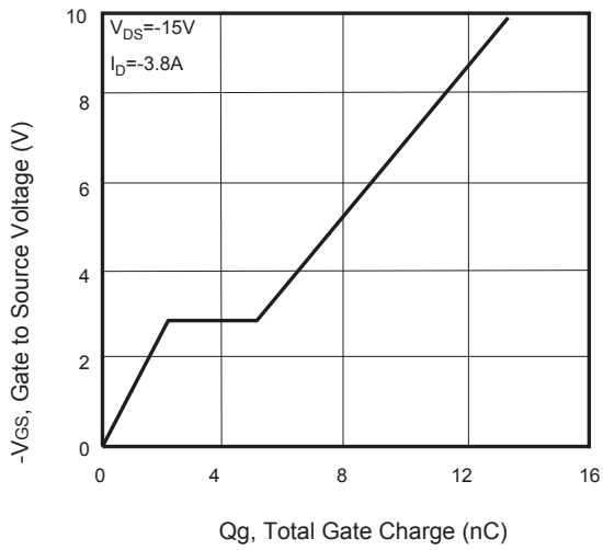
Figure 7. Gate Charge
