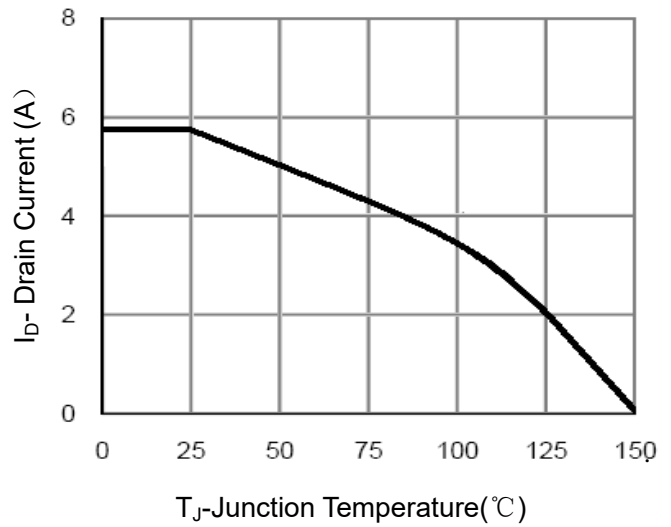
Figure 2 Drain Current
