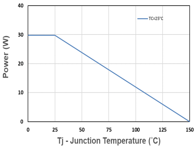
Figure 9. Power Dissipation
