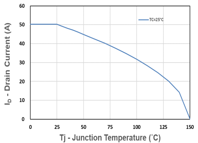
Figure 10. Drain Current
