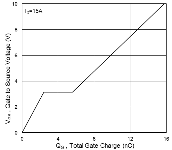
Fig.4 Gate-Charge Characteristics
