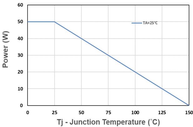
Figure 9. Power Dissipation
