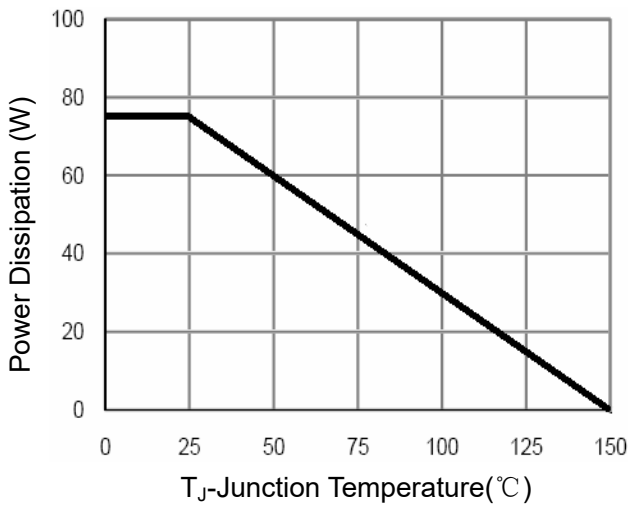
Figure 9 Power De-rating
